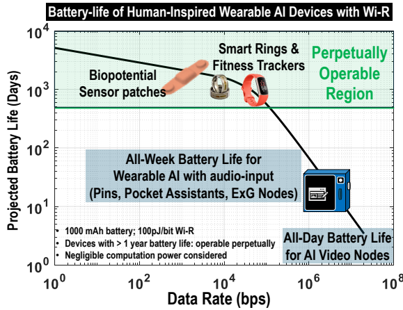
Figure 3: Projected battery life of wearables with respect to data rate using Wi-R [29]. Power consumption is calculated using a survey of literature and commercial devices [29].
